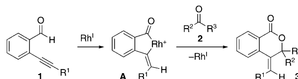
Scheme 1. Rhodium-catalyzed enantioselective [4+2] annulation of 2-alkynylbenzaldehydes 1 with carbonyl compounds 2 .
