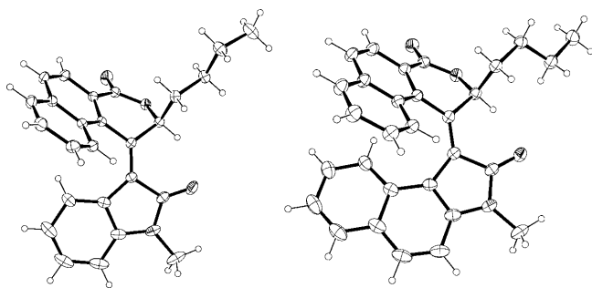
Figure 1. ORTEP diagrams of tetrasubstituted helical alkenes ( \pm )- 4ha (left) and ( \pm )- 4he (right) drawn at the 30% probability level.
